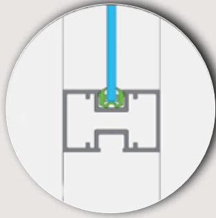
enkele beglazing
